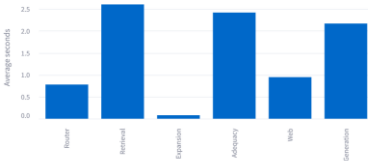
Average latency by pipeline stage
